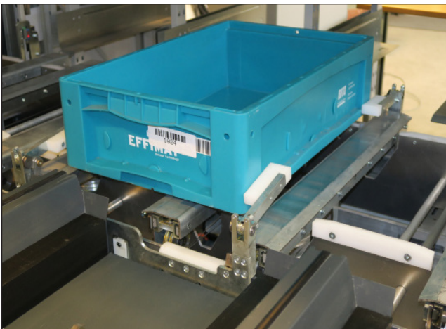
Intelligent Box Mover Technology allows boxes to be moved horizontal
