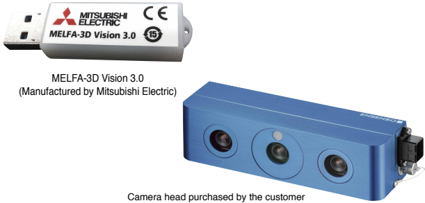
MELFA-3D Vision 3.0 (Manufactured by Mitsubishi Electric) Camera head purchased by the customer Manufacturer: ENSENSO GmbH. (Supplier: IDS Imaging Development Systems GmbH.) For more details, please refer to the IDS website. https://en.ids-imaging.com/ensenso-3d-camera-n-series.html
