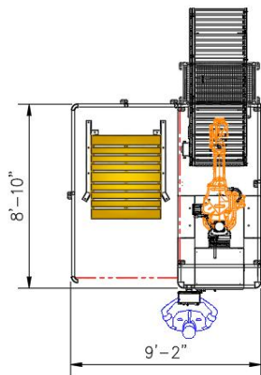
SINGLE LAYOUT
