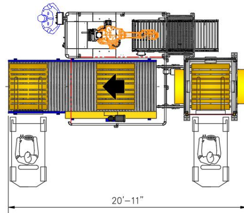
CUBE+ LAYOUT
